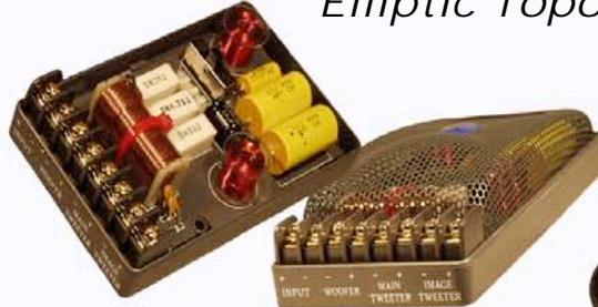
SatNet-480 Elliptic 2-way 4th order
